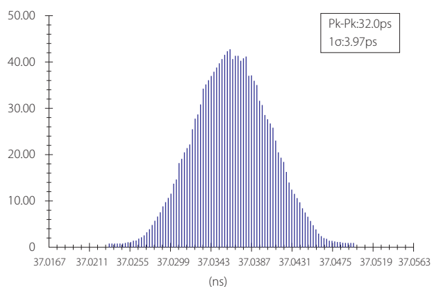
Period Jitter SCV-3225 27.000MHz
