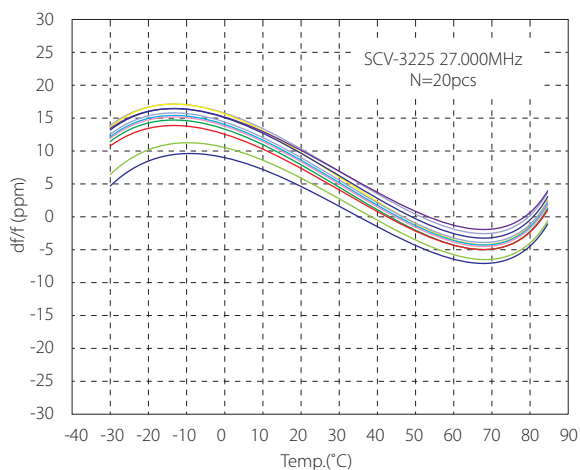
Frequency Temperature Characteristics
