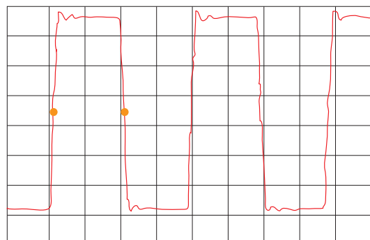
Output wave SCV-3225 27.000MHz
