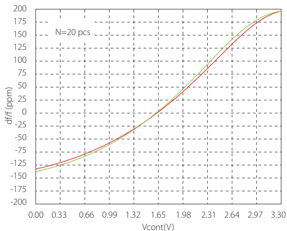
VOXO Characteristics of SCV-3225 27.000MHz
