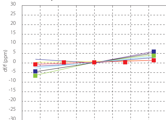
Vdd stability of SCV-3225 27.000MHz
