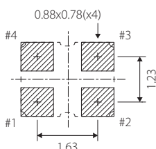
Land Pattern(REFERENCE)
