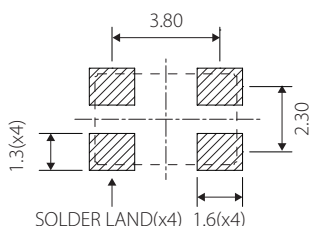
Land Pattern(REFERENCE)
