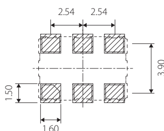
Land Pattern(REFERENCE)
