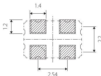
Land Pattern(REFERENCE)
