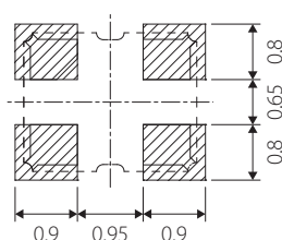
Land Pattern(REFERENCE)
