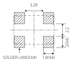
Land Pattern(REFERENCE)
