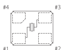
Land Pattern(REFERENCE)
