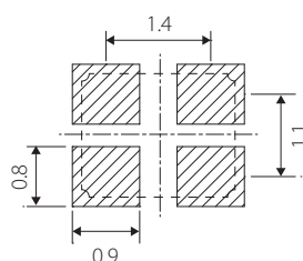
Land Pattern(REFERENCE)
