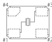
Land Pattern(REFERENCE)
