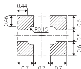
Land Pattern(REFERENCE)
